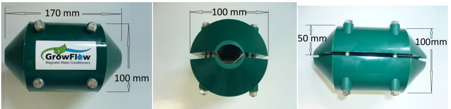
GrowFlow Magnetic Water Conditioner 25mm / 1" GF25 Unit Weight 2.2
