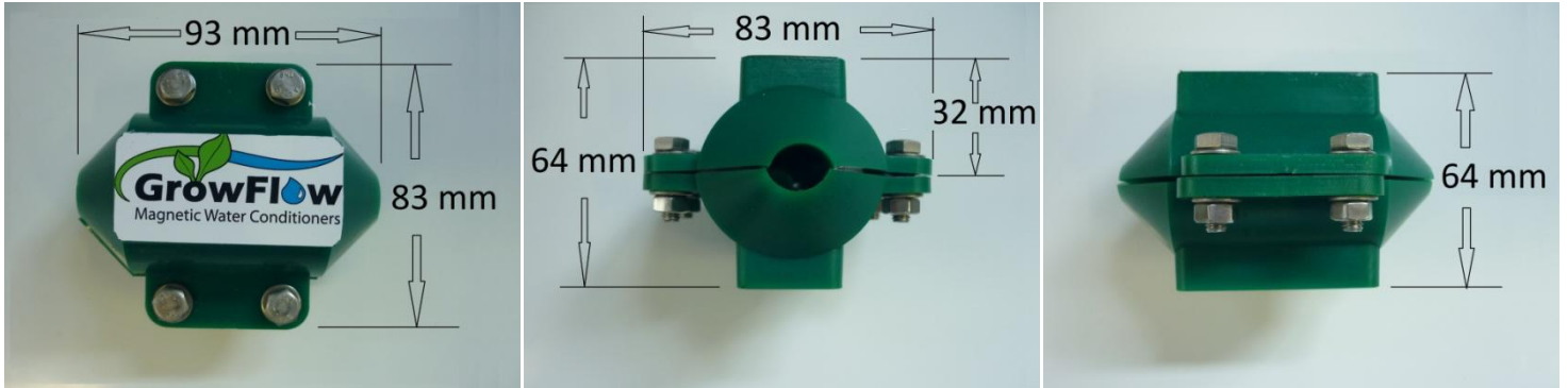
GrowFlow Magnetic Water Conditioner 12.5mm / ½" GF12.5 Unit Weight 400 gms
